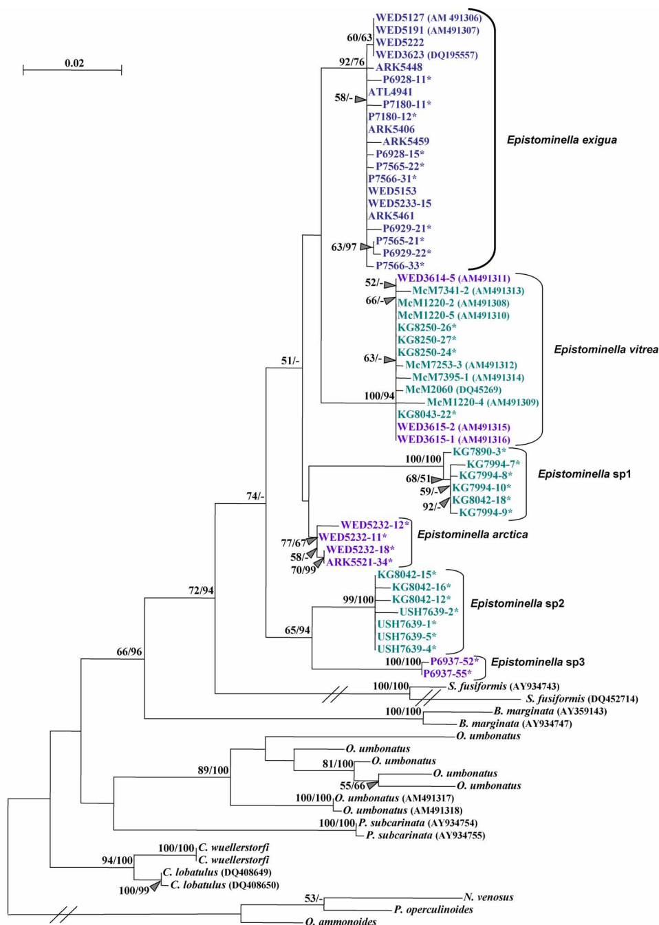
FIGURE 1. Phylogenetic tree inferred from SSU rDNA sequences showing the position of E. exigua among other Epistominella species and the lack of differentiation between populations of E. exigua from different regions. This tree has been obtained using the ML method with 1000 bootstrap replicates. The support values at internal nodes correspond to ML (left) and Bayesian (right) analyses. Only values over 50% were indicated. Within the genus Epistominella , first letters of the Epistominella sequence names indicate their geographical origin (ARK: Arctic, WED: Weddell Sea, ATL: North Atlantic, P: Pacific, McM: Mc Murdo Sound, USH: Ushuaia, KG: King George Island) and colour indicates a range of depths (purple: 0-200 m; green: 200–1200 m; dark blue: >1200 m). New sequences are indicated by a star (*).
