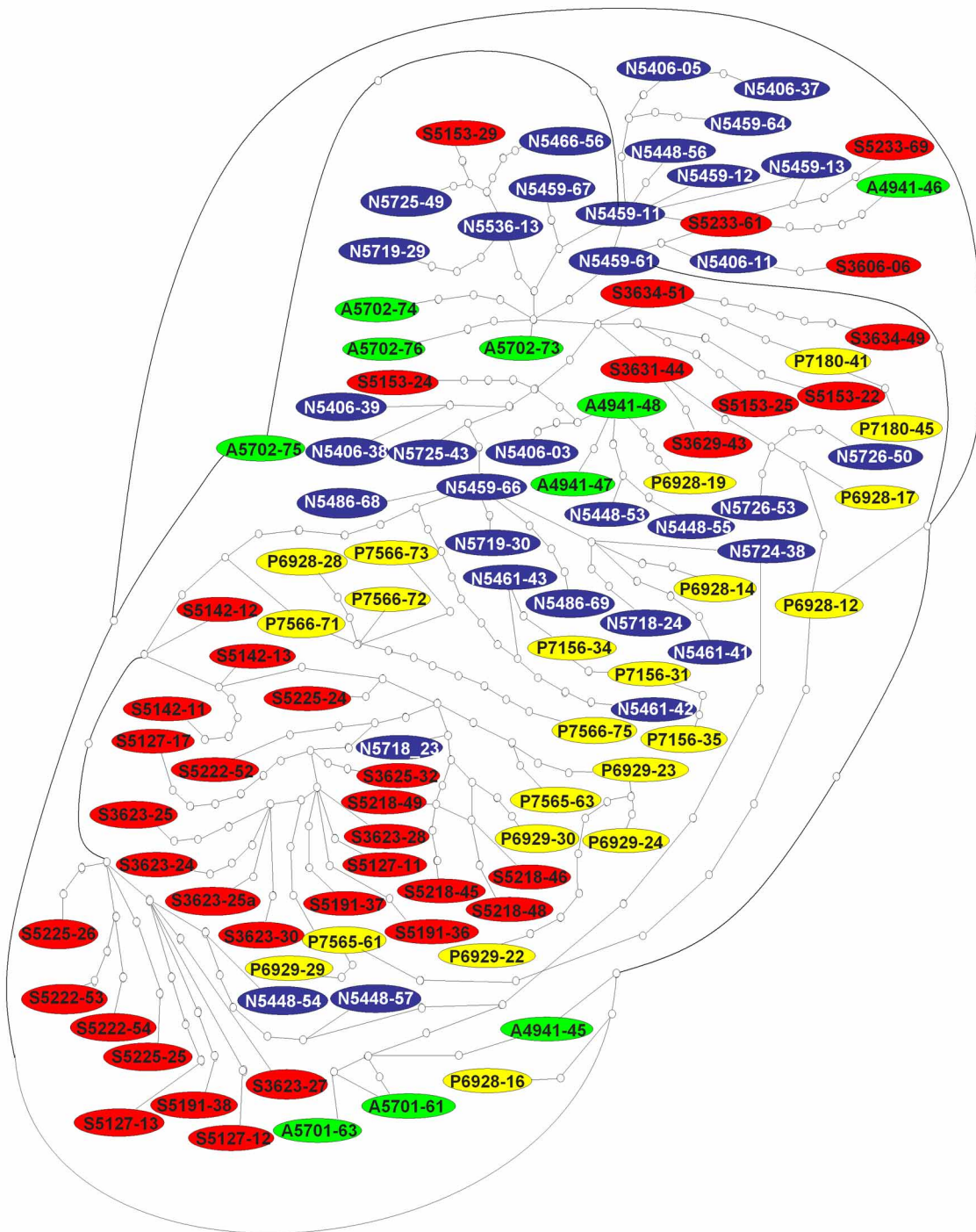
FIGURE 3. ITS sequences network performed by TCS software: schema of genetic relationships between each haplotype (1 node represents a difference of 1 nucleotide or indel). Geographic origin of haplotypes is indicated by the color of the boxes: yellow for Pacific, red for Antarctic, blue for Arctic and green for North Atlantic.
