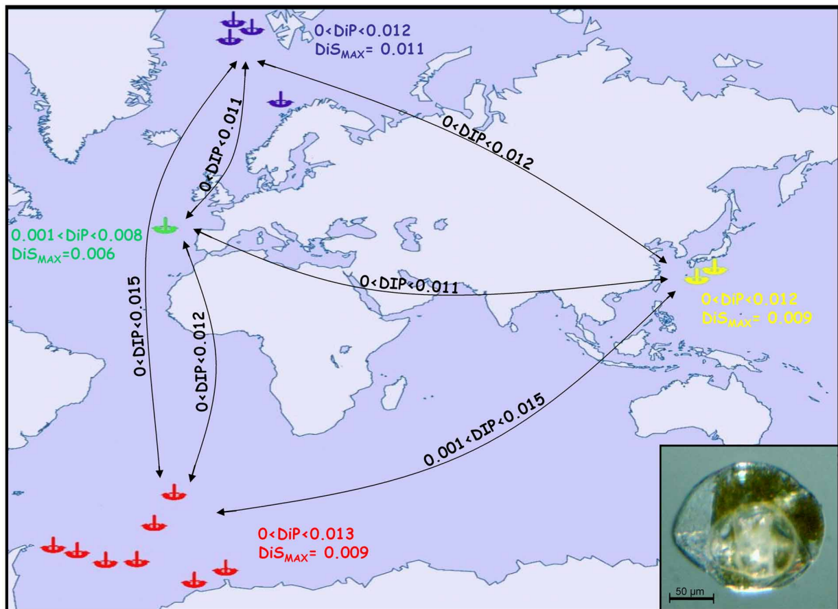
FIGURE 2. In Background. Map with position of Epistominella exigua sampling sites (red anchors for Antarctic, green for Atlantic, blue for Arctic and yellow for Pacific). In Foreground. E. exigua ITS rDNA sequence divergences. Minimum and maximum values of divergences within each geographic population (DiP) as well as maximum values of intraspecimen divergences (DiS) are indicated in color according to the sampling sites. Minimum and maximum values of divergences between each geographic population (DIP) are indicated above black arrows. Inset. Epistominella exigua specimen collected off Japan.
